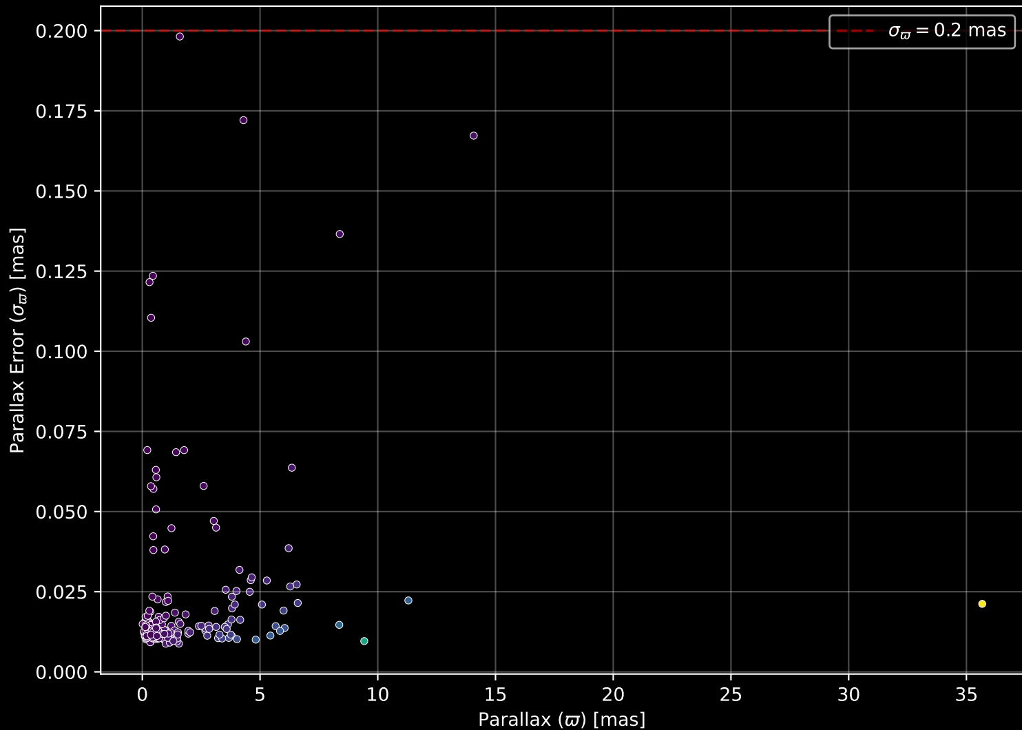
APOGEE DR17 Field: [N2243-S] Parallax Quality (n= 213)
