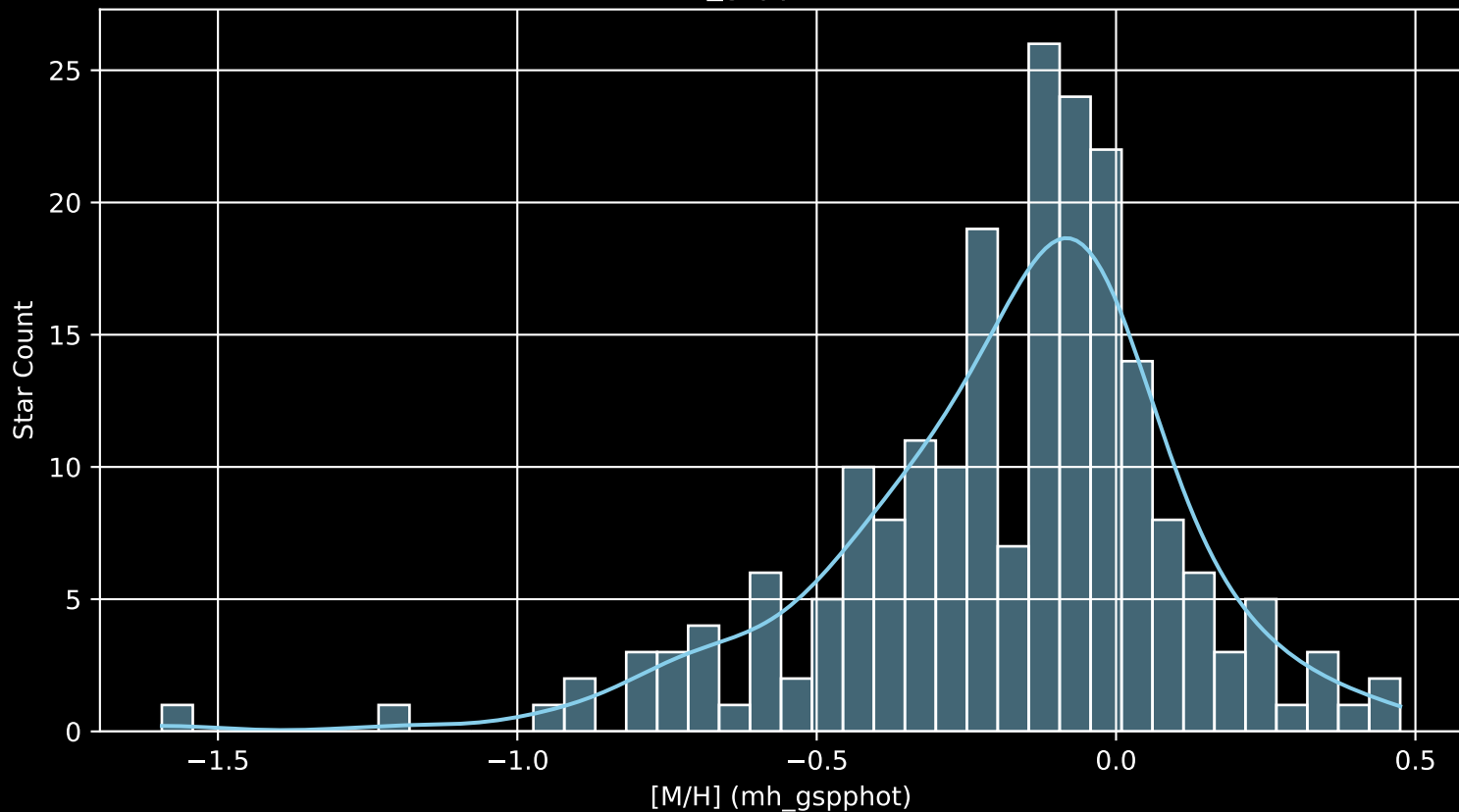
APOGEE DR17 Field: [N2243-S [M/H] (mh_gspphot) (n= 209)
