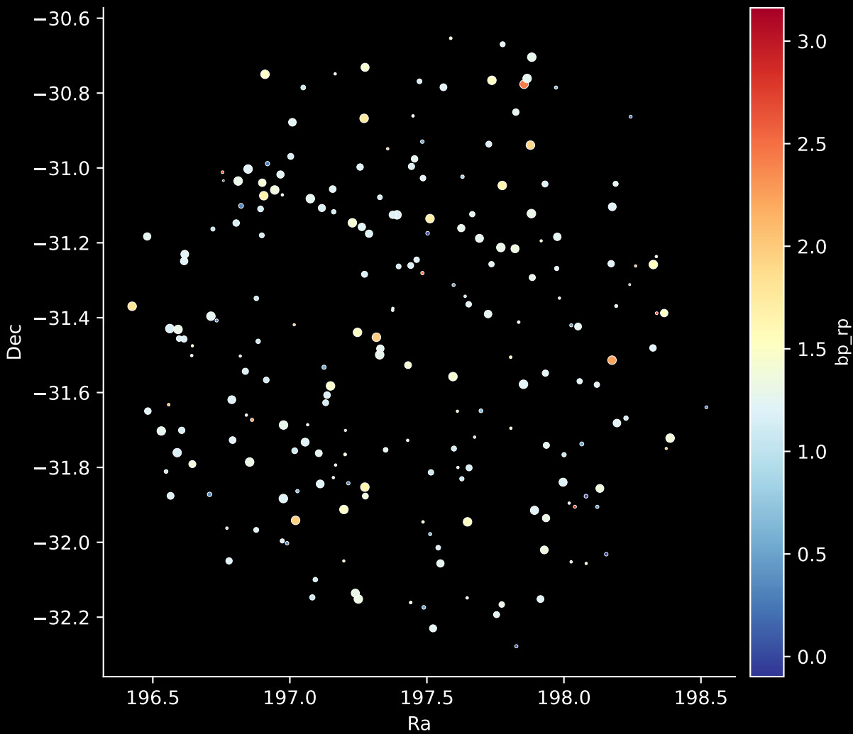
APOGEE DR17 Field: [N2243-S] Stars: 213
