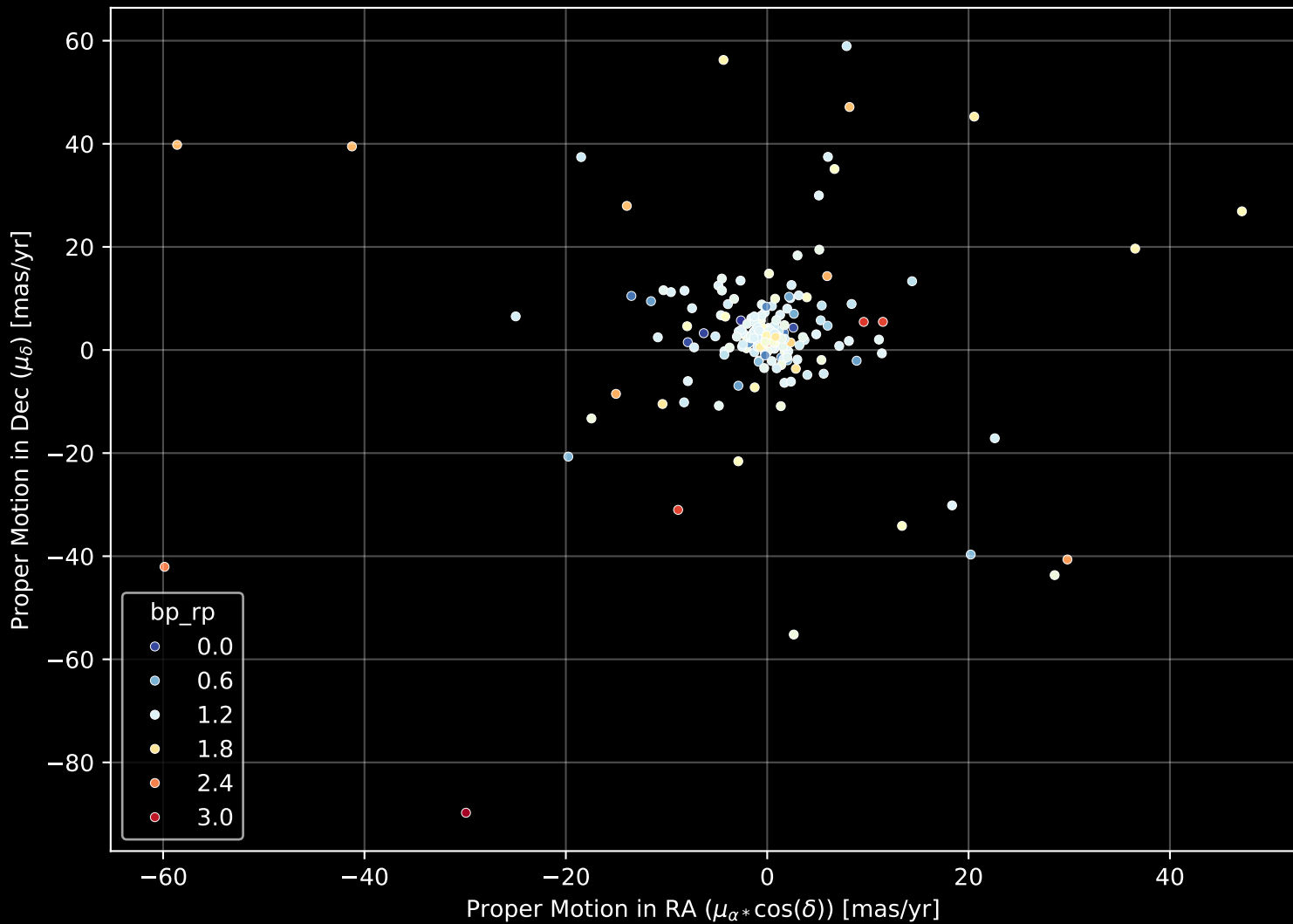
APOGEE DR17 Field: [N2243-S] Proper Motion Diagram (n= 213)
