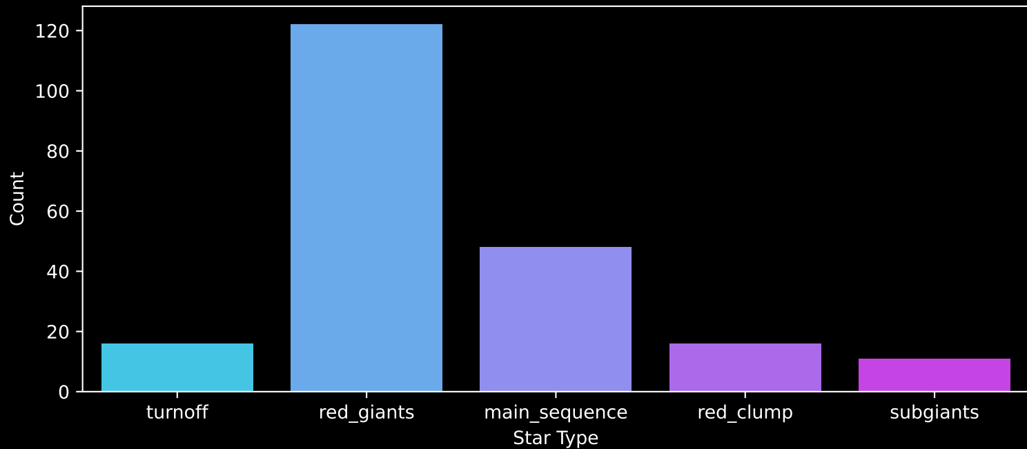
APOGEE DR17 Field: [N2243-S] Count plot of Star Type
