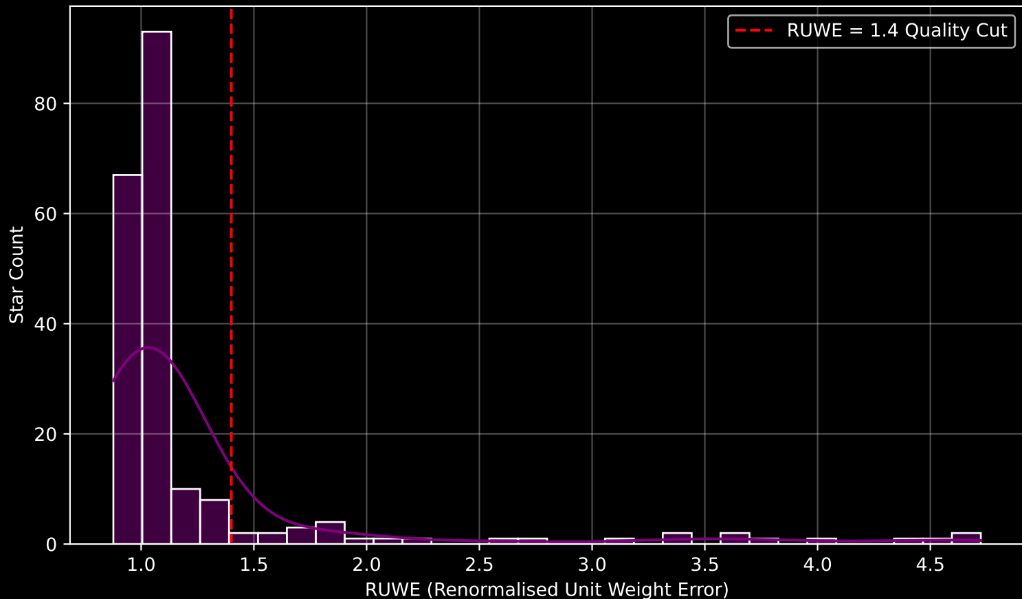
GAPOGEE DR17 Field [N2243-S] RUWE Distribution (n= 205)
